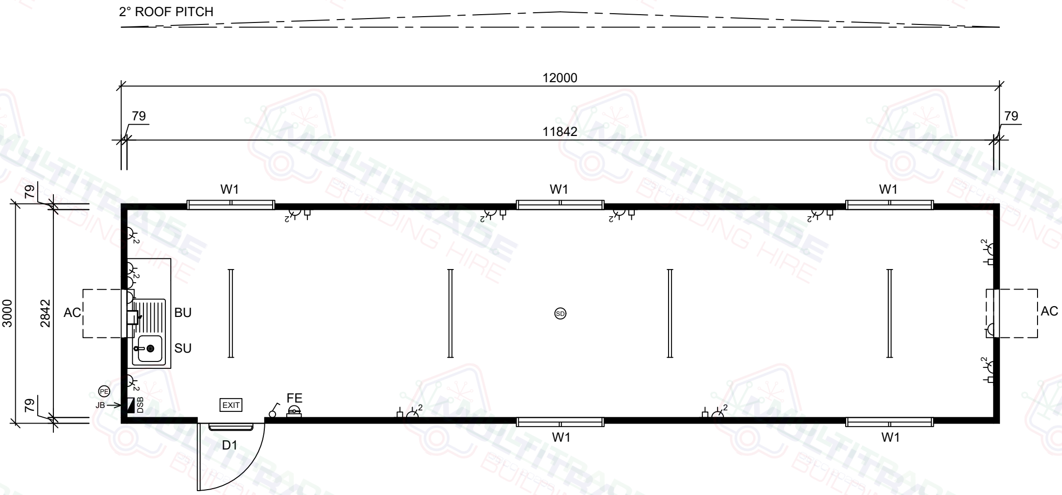
12.0x3.0m Crib Room - Floor Plan
